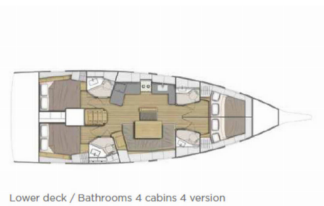
Lower deck / Bathrooms 4 cabins 4 version
